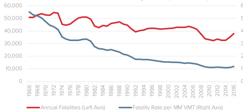
Annual Motor Vehicle Fatalities & Fatality Rates (1966-2016)
