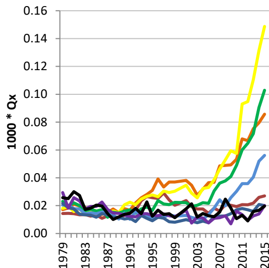
Accidental Poisoning Qx's by Age, U.K.
